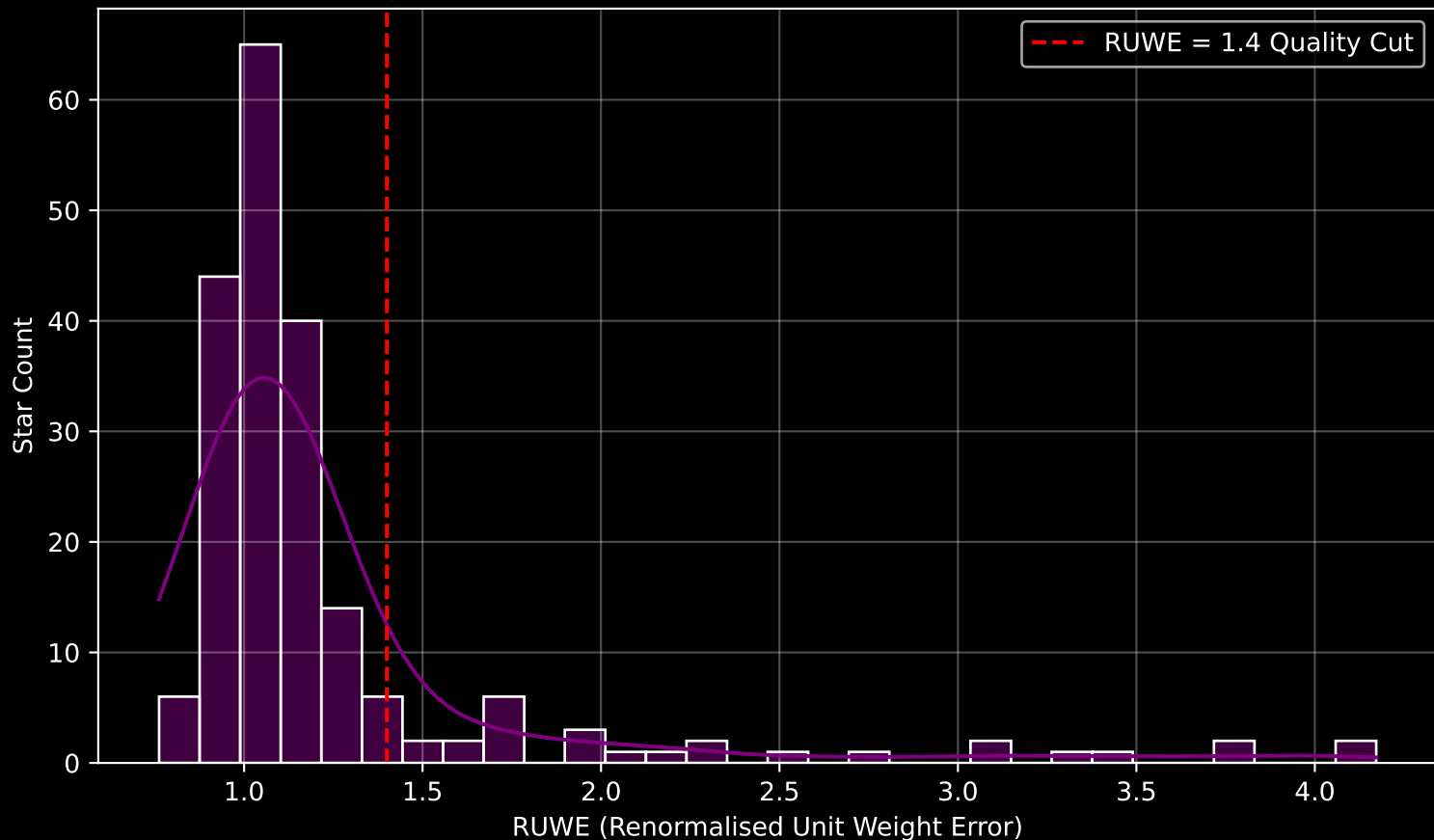
GAPOGEE DR17 Field [265-35-O_TESS] RUWE Distribution (n= 202)
