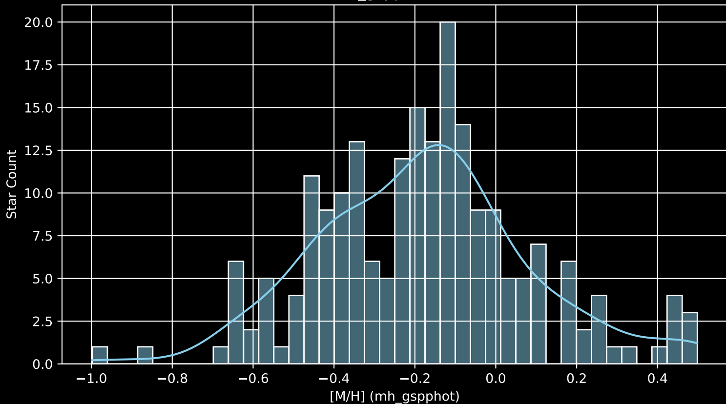
APOGEE DR17 Field: [265-35-O_TESS [M/H] (mh_gspphot) (n= 206)
