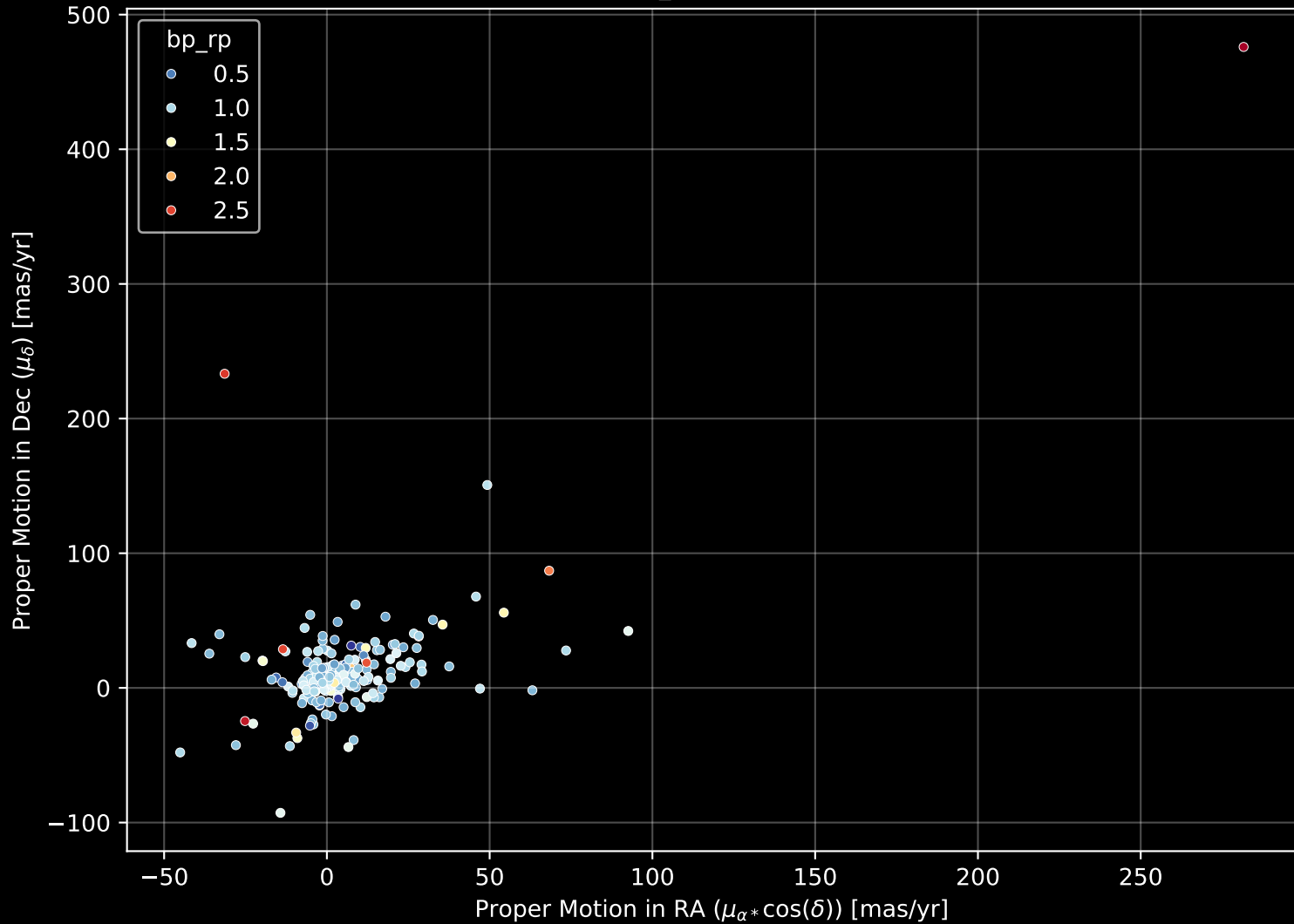
APOGEE DR17 Field: [265-35-O_TESS] Proper Motion Diagram (n= 209)
