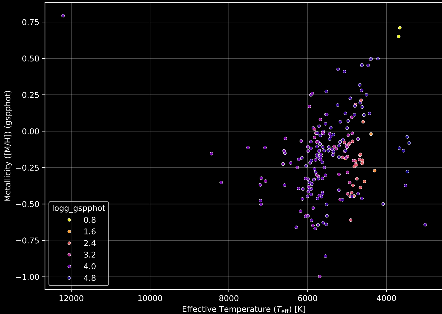
APOGEE DR17 Field: [265-35-O_TESS] Stellar Population Parameters (n= 209)
