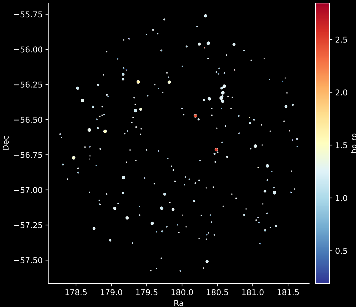
APOGEE DR17 Field: [265-35-O_TESS] Stars: 209
