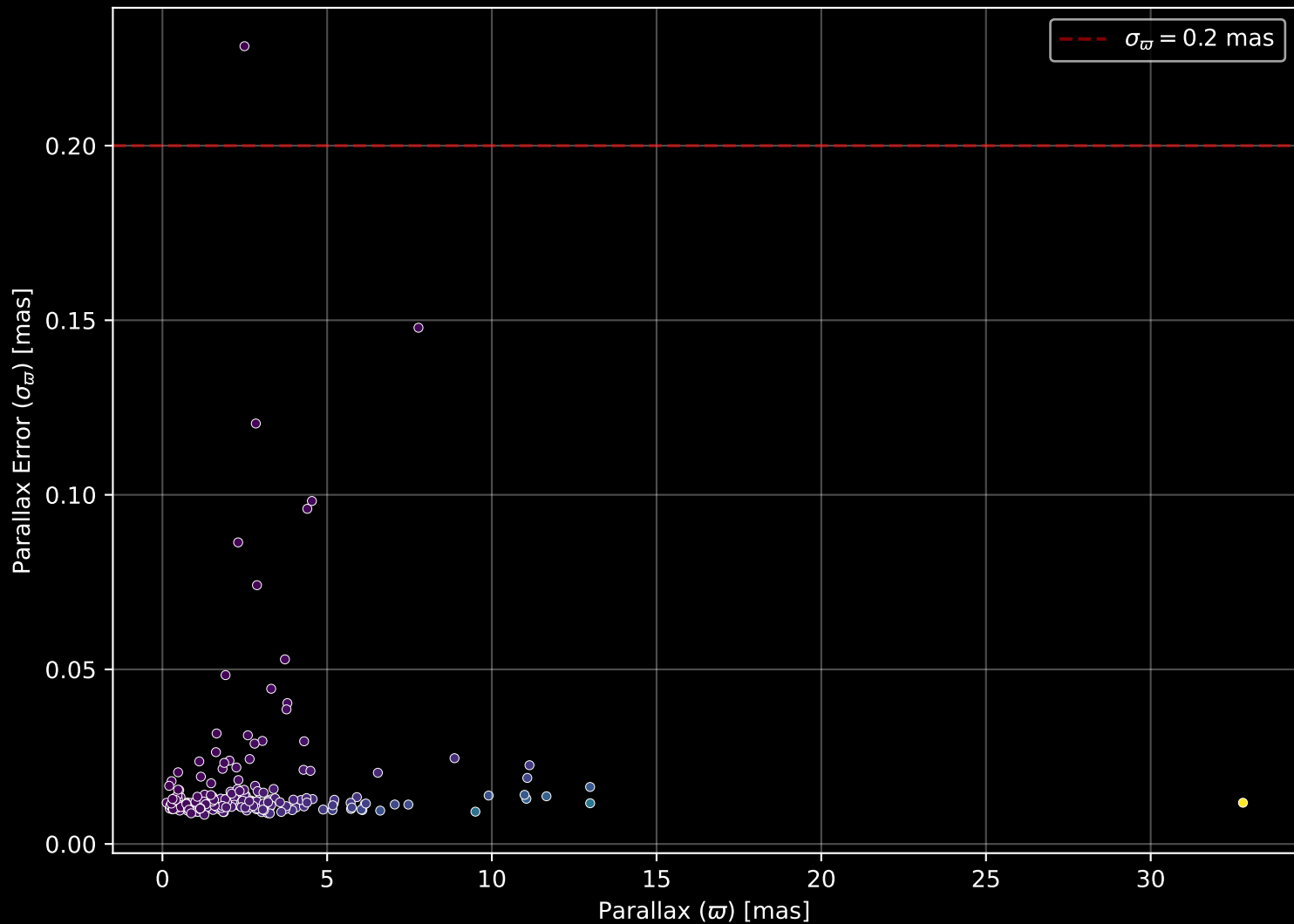
APOGEE DR17 Field: [265-35-O_TESS] Parallax Quality (n= 209)
