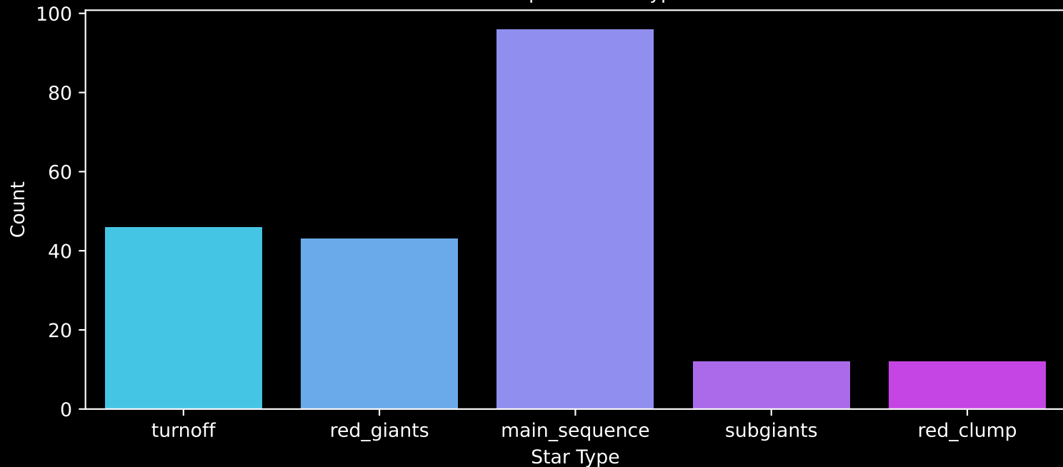
APOGEE DR17 Field: [265-35-O_TESS] Count plot of Star Type
