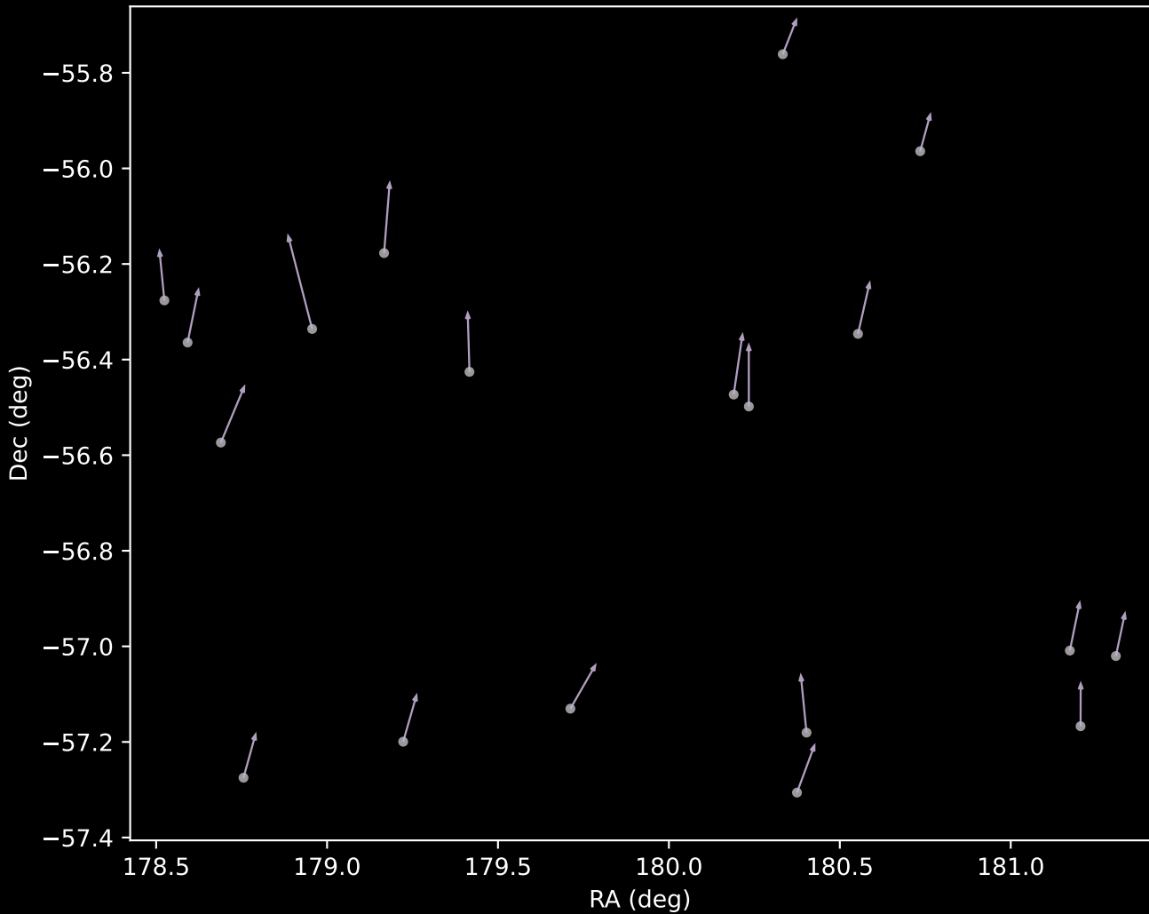
APOGEE DR17 Cluster 9 Proper Motion Vectors (n=19)
